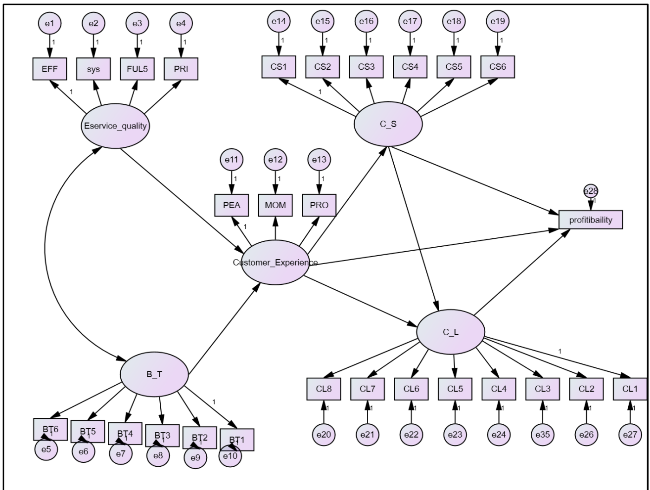
Figure 2. Path model
